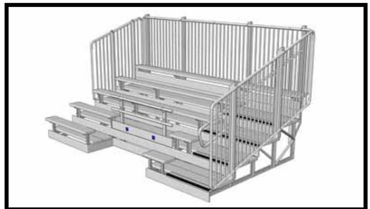
ADA Series NB-0515AADA 5 Row 15' long with 34 seats + 2 Handicap seats center aisle with anodized handrail and optional vertical picket guardrail.
