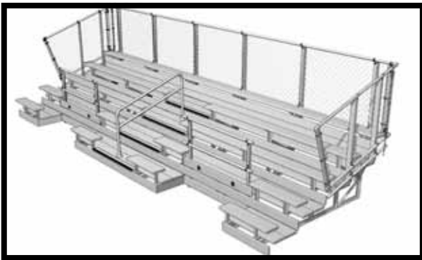
ADA Series NB-0527AADA 5 Row 27.5' long with 58 seats + 5 Handicap seats center aisle with anodized handrail and chainlink guardrail.
